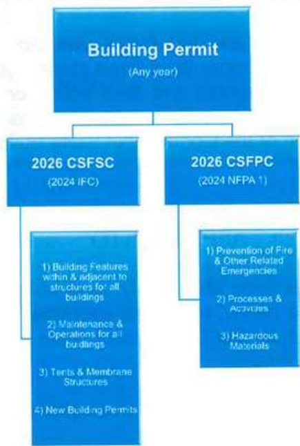
(Add) Figure 102.1 Connecticut State Fire Safety Code Application Flow Chart.
